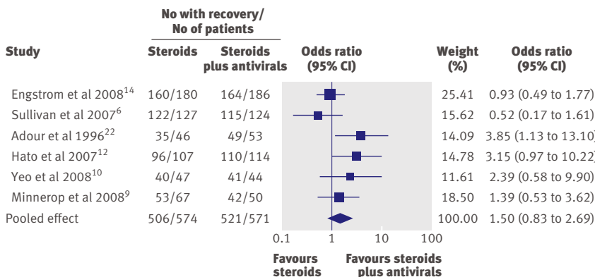
Fig 2 | Forest plot of the six included studies ordered according to Jadad score (highest quality to lowest) showing the odds ratio estimates and their 95% confidence intervals. The pooled estimate is based on a random effects model
