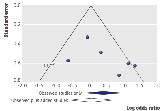
Fig 5 | Funnel plot of the six included studies (solid circles) and two added studies (open circles) based on a trim and fill algorithm. The pooled odds ratio and 95% confidence interval based on the six included studies (solid diamond) and following the addition of the extra studies (open diamond) are shown
