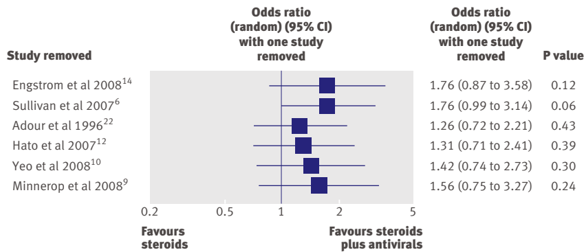
Fig 4 | Forest plot of a one study removed analysis showing the odds ratio estimate and 95% confidence interval if the study specified in the “Study removed” column is not included
