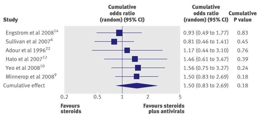
Fig 3 | Cumulative forest plot of the six included studies, ordered according to study quality (highest quality to lowest)
